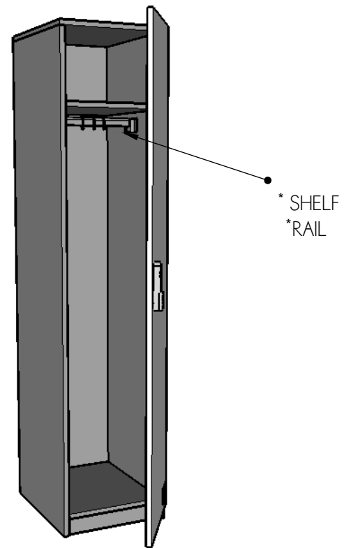
MODEL A * ADDITIONAL SHELF * RAIL WITH HOOKS
