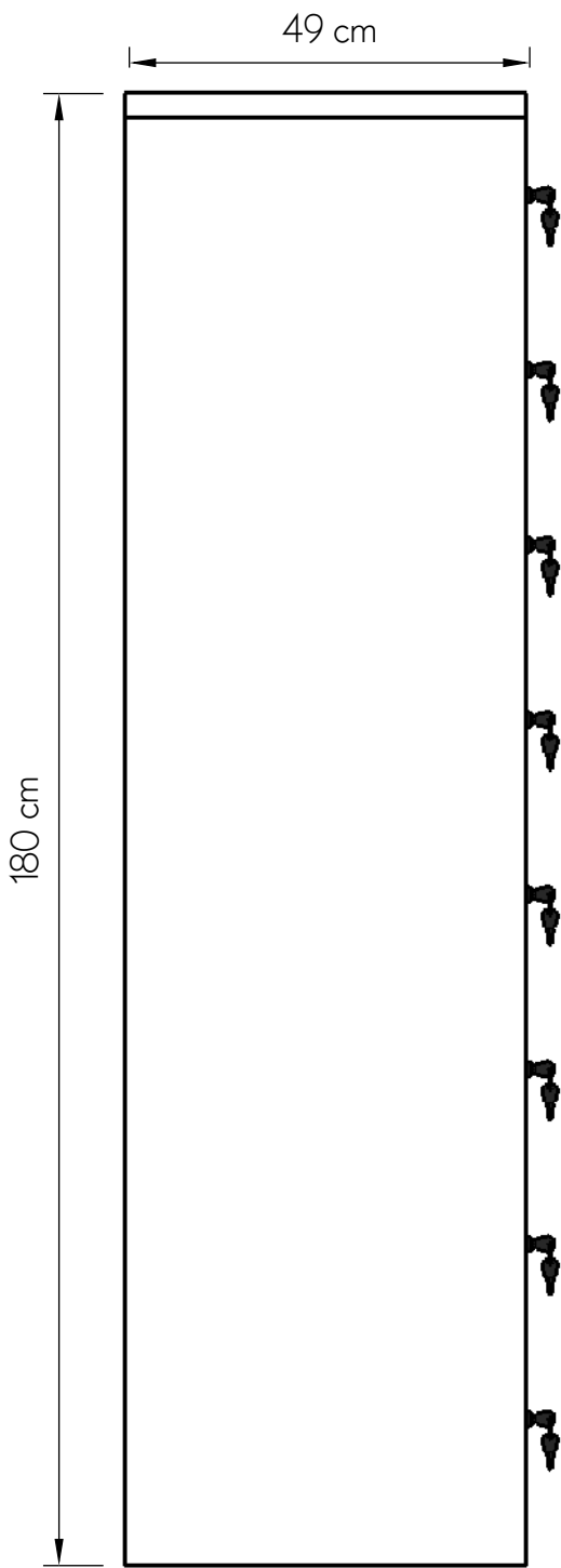
SIDE VIEW
